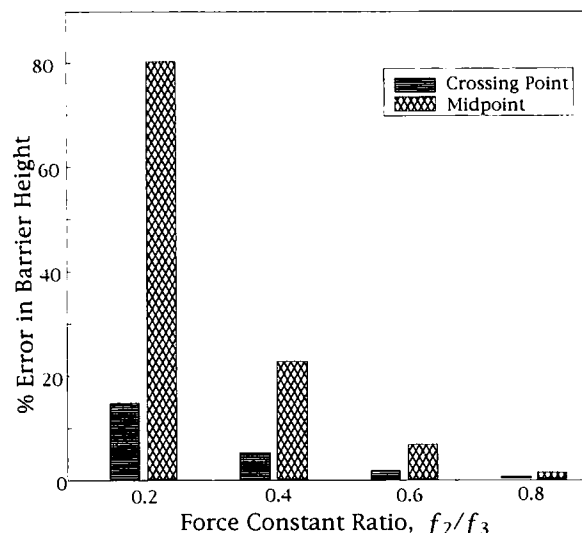
Fig. 5. Bar graph showing the difference between \Delta G^* , the inner-shell activation energy given by Eq. (14a), and either \Delta G_{\text{cp}} , the inner-shell energy required to reach the configuration crossing point shown in Fig. 4 and given by Eq. (21), or \Delta G_{\text{mp}} , the inner-shell energy required to reach the midpoint configuration shown in Fig. 4 and given by Eq. (19).
